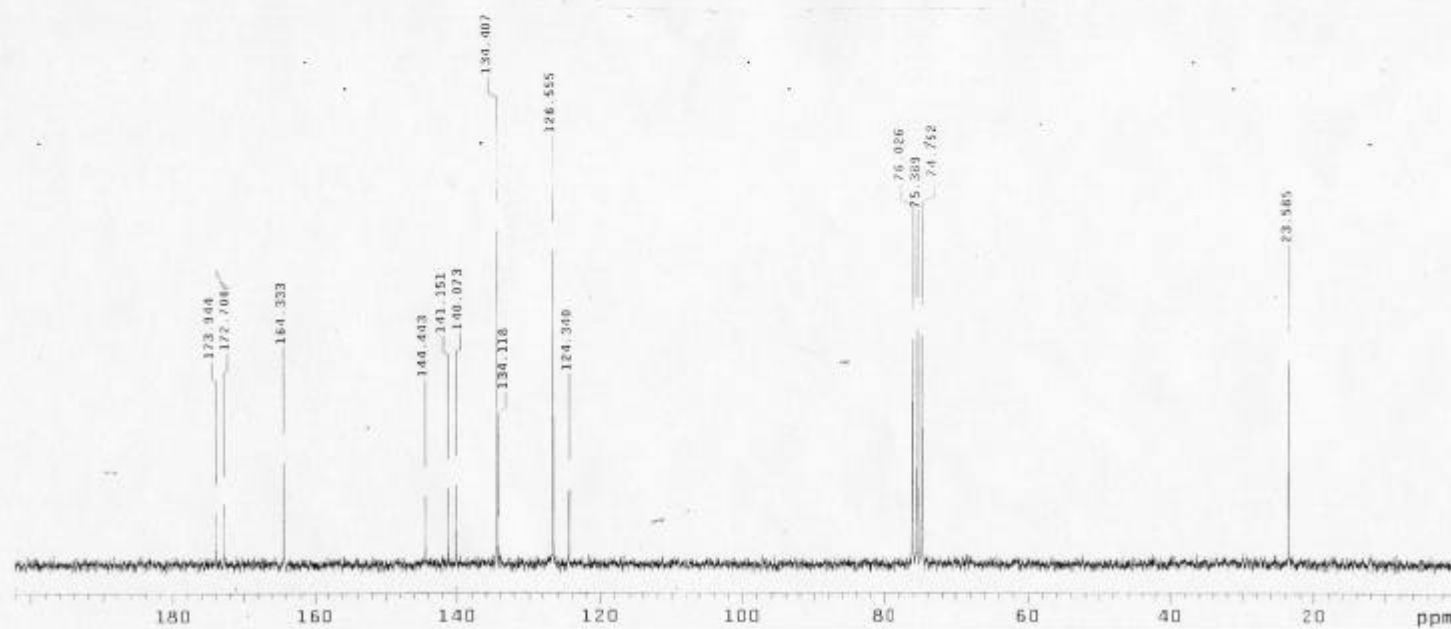
2-methyl-6,7-dibromoquinoline-5,8-dione (2c)
