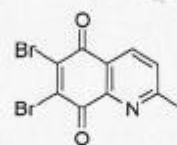
2-methyl-6,7-dibromoquinoline-5,8-dione (2c)
