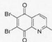
2-methyl-6,7-dibromoquinoline-5,8-dione (2c)
